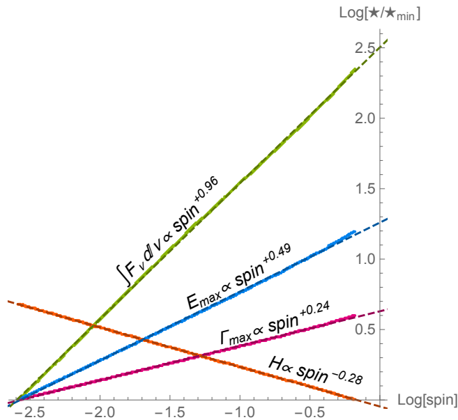
Figure 11. The \star is a place holder that represents the maximum Lorentz factor, maximum electric field, gap width, and photon energy flux. Each physical quantity is normalized to its minimum value and then plotted with respect to the spin of the BH on a log-log scaling.
