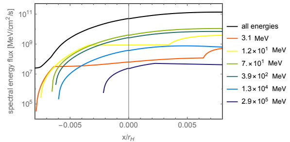
Figure 4. The outgoing photon energy flux as a function of position inside of the gap. This result is for a maximally spinning BH of mass 10^7 M_\odot with a magnetic field strength of 10^4 Gauss and an ambient energy density of 10^6 ergs/cm 3 . The x -axis has been normalized by the BH radius.
