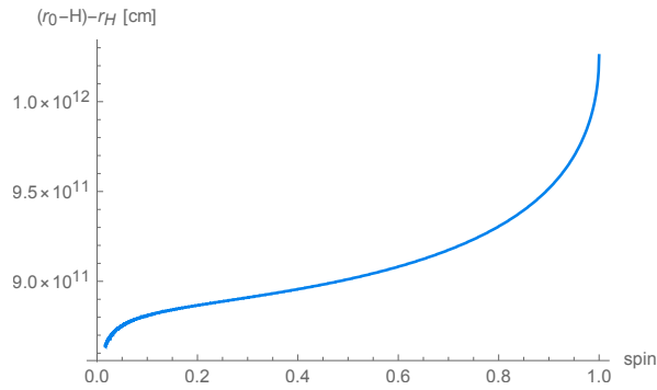
Figure 10. The distance between the BH horizon and the inner edge of the gap as a function of spin for a BH of mass 10^7 M_\odot with a magnetic field strength of 10^4 Gauss and an ambient energy density of 10^6 ergs/cm ^3 .
