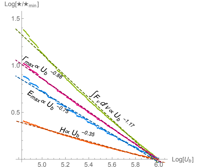
Figure 12. The \star is a place holder that represents the maximum Lorentz factor, maximum electric field, gap width, and photon energy flux. Each physical quantity is normalized to its minimum value and then plotted with respect to the background energy density on a log-log scaling.
