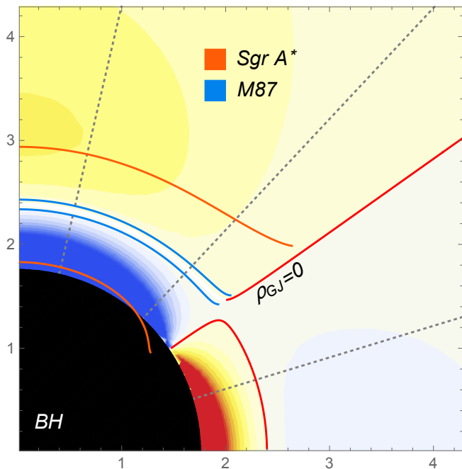
Figure 16. The BH radius of a maximumly spinning BH has been set to one and the gap widths have been left to scale. M87 has a luminosity of 2.7 \times 10^{42} ergs/s, mass of 10^{9.5} M_{\odot} , a spin of 0.65, and a magnetic field of 15 G. Sgr A* has a luminosity of 10^{37} ergs/s, mass of 10^{6.6} M_{\odot} , a spin of 0.65, and a magnetic field of 30 G.
