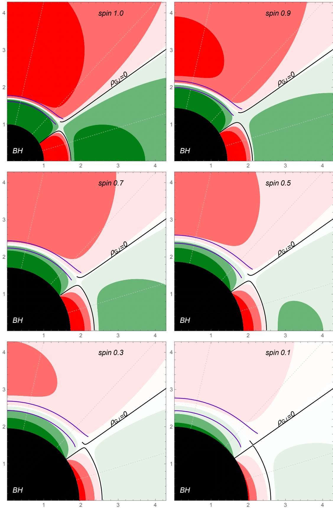
Figure 13. Gap width increased by an order of magnitude. for a maximally spinning BH, the radius is set to one. The plasma density is displayed in red and green which correspond to positive and negative charge densities, respectively. It can be seen that as the BH's spin decreases the gap width increase and the plasma density around the gap decreases.
