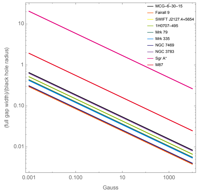
Figure 15. The curve for Sgr A* is at the top and followed by M87. Next is MCG-6-30-15 and NGC 3783. They are followed by 1H0707-495. Next Mrk 79, Mrk 335, and SWIFT J2127.4+5654 are clustered together. They are followed by NGC 7469 and Fairall 9. The values for mass, spin, and energy density in Eq. 36 are listed in Table II.
